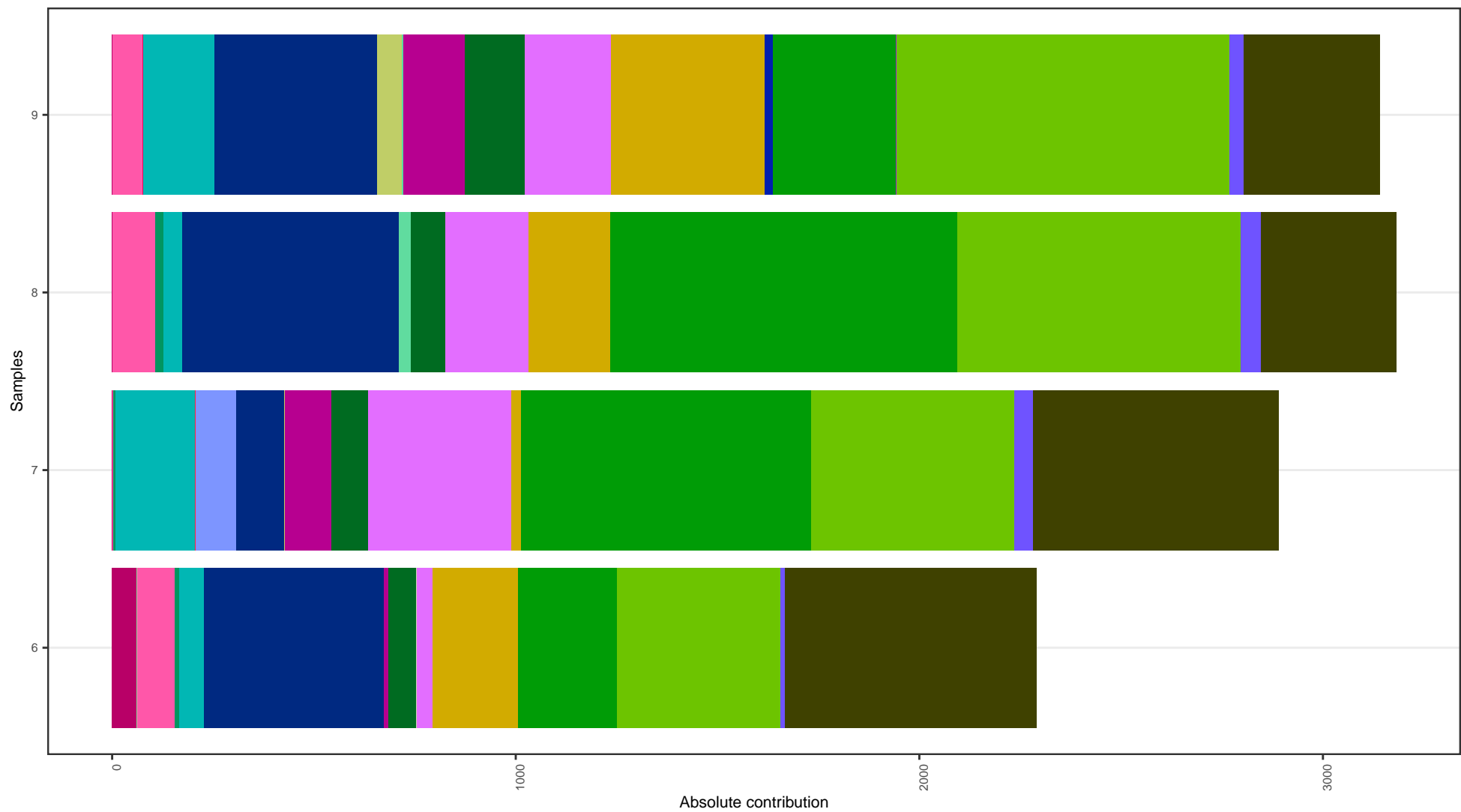
Absolute and Relative Contributions of elementary signatures to mutational profiles
