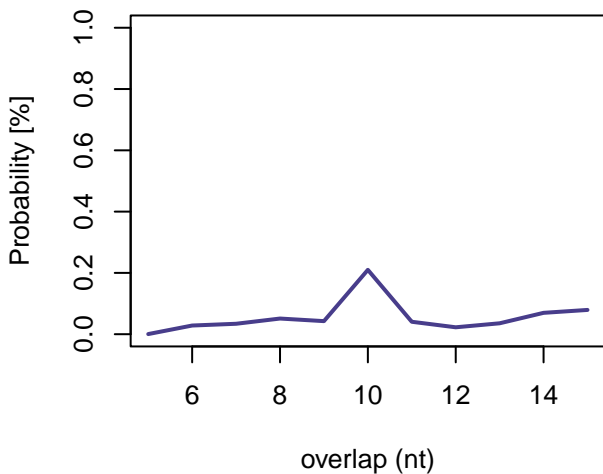
Overlap probabilities
