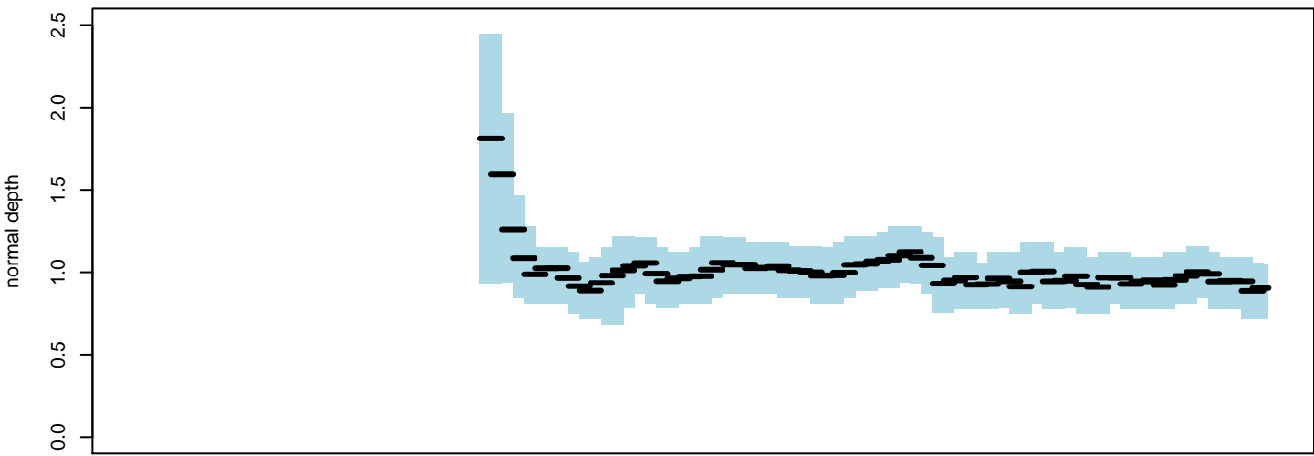
raw chr22
