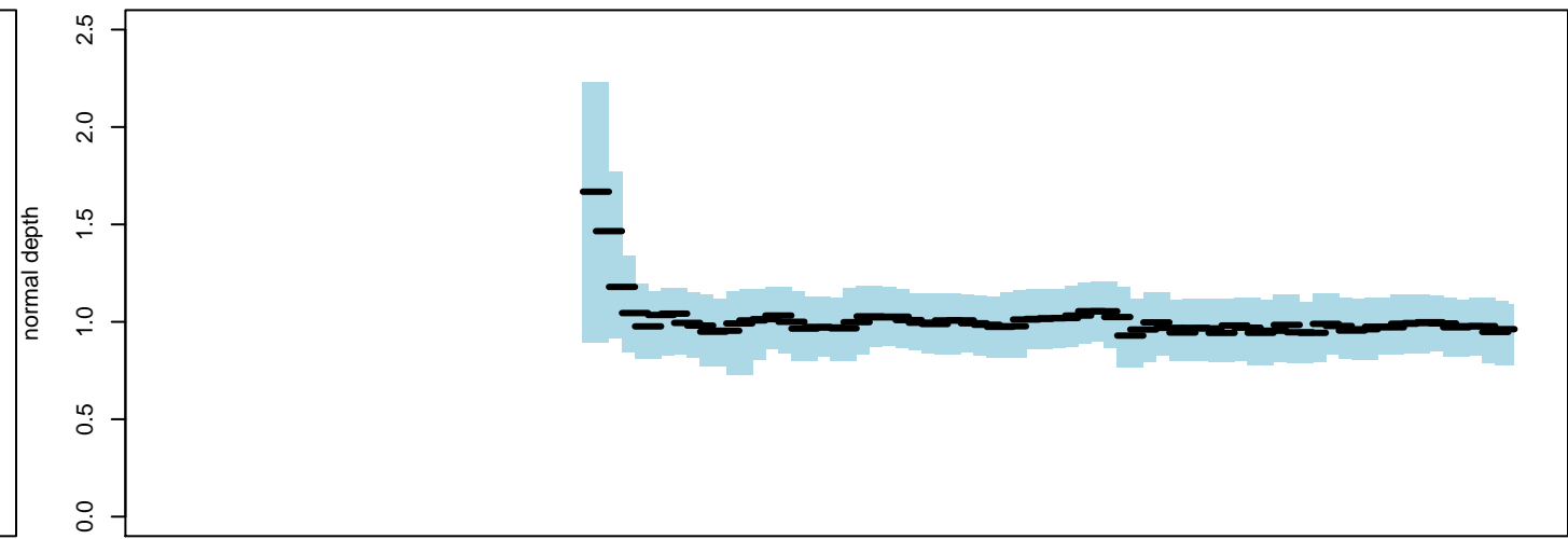
normalized chr22
