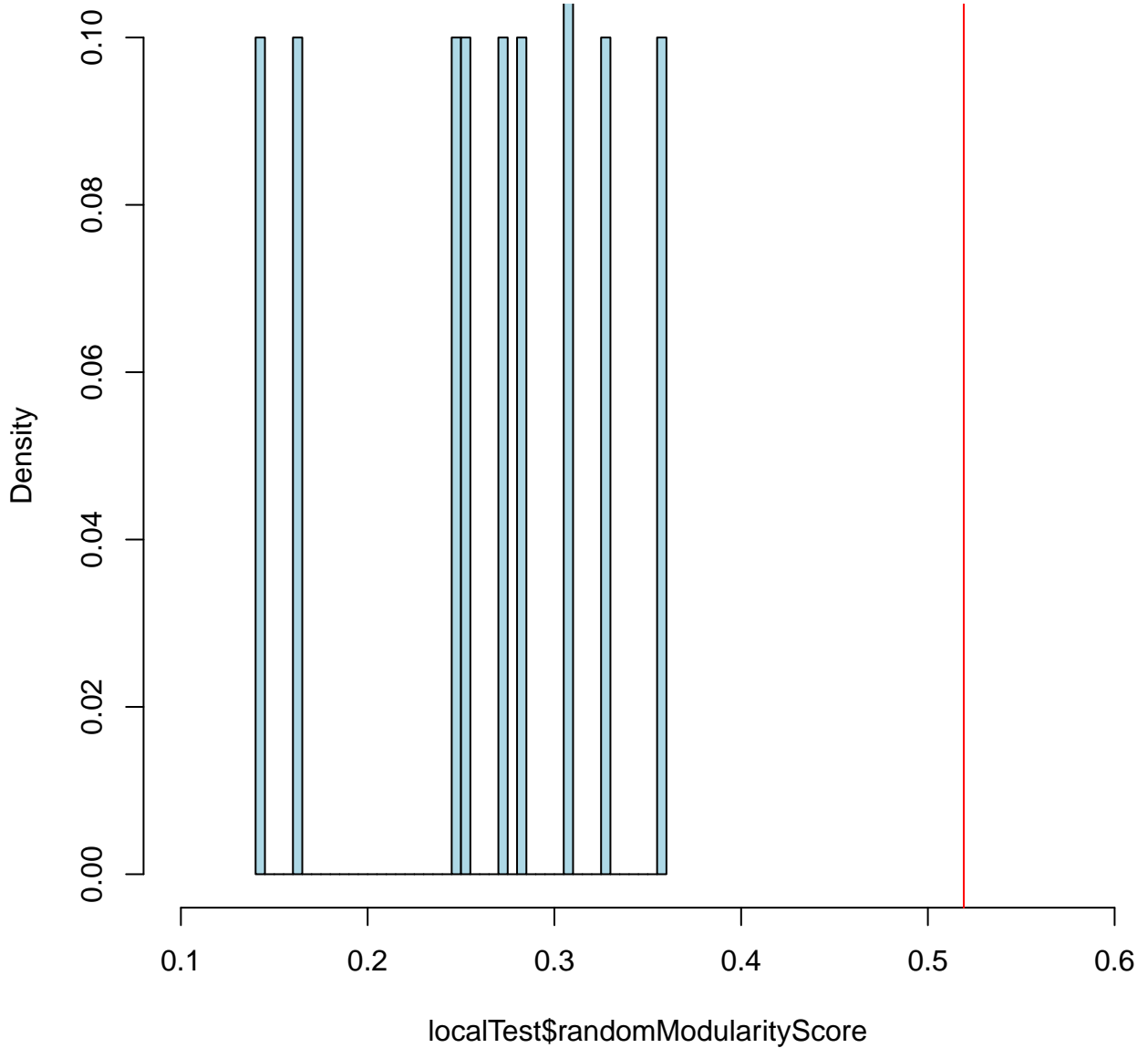
Histogram of localTest$randomModularityScore
