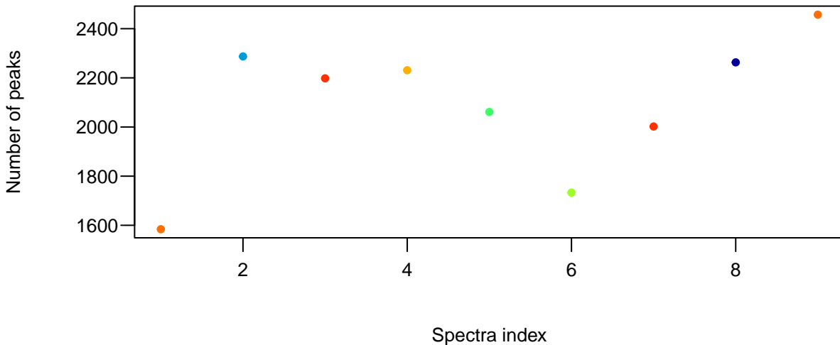
Number of peaks per spectrum
