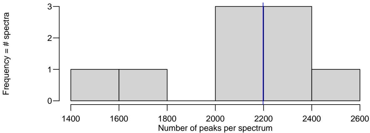
Number of peaks per spectrum
