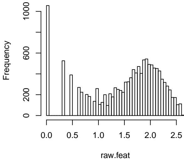
RawData Log10(NumFeat)
