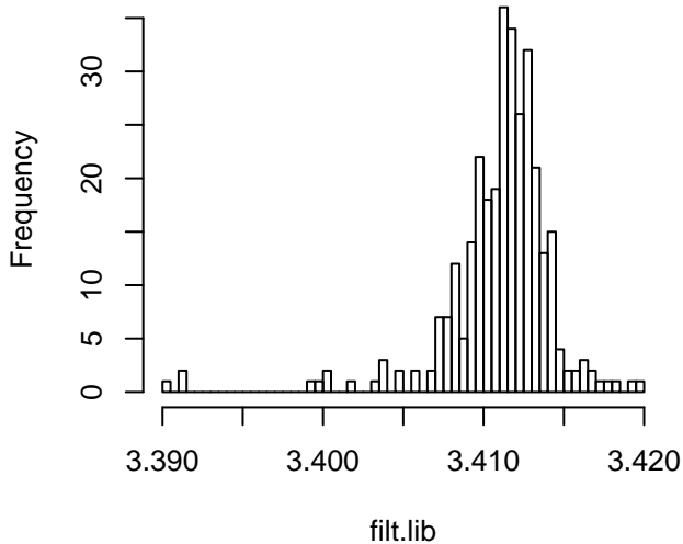
FiltData Log10(LibSize)
