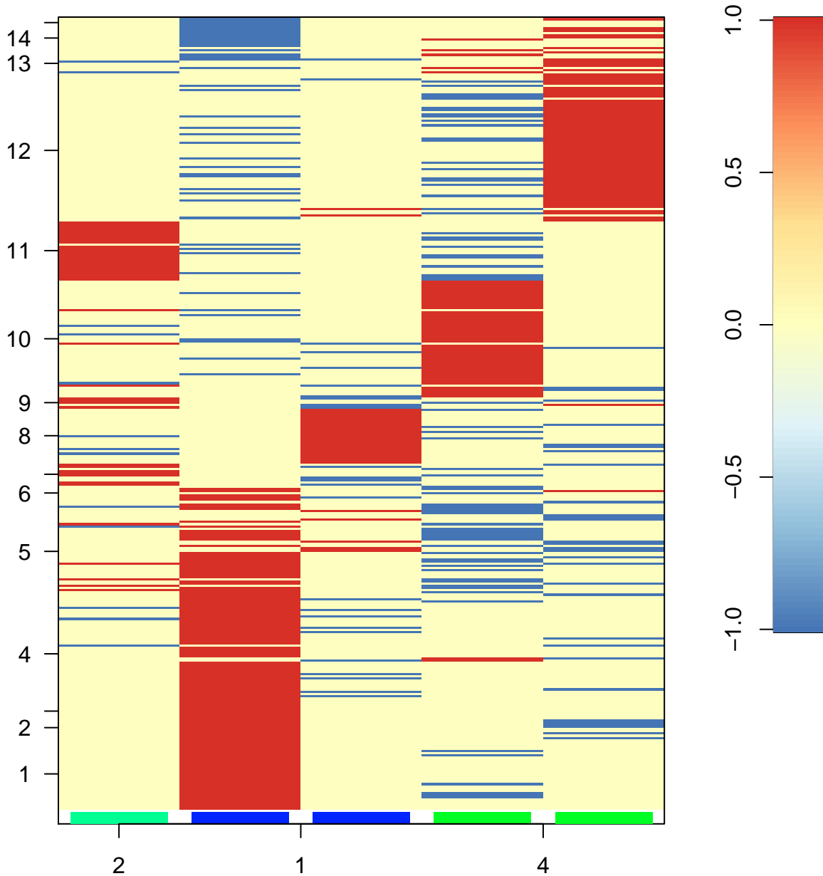
Binarized expression profile of each gene
