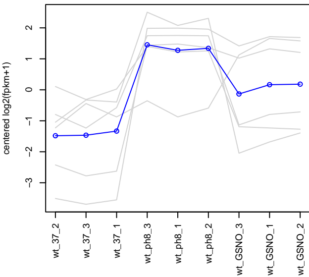
subcluster_1_log2_medianCentered_fpkm.matrix, 6 tran
