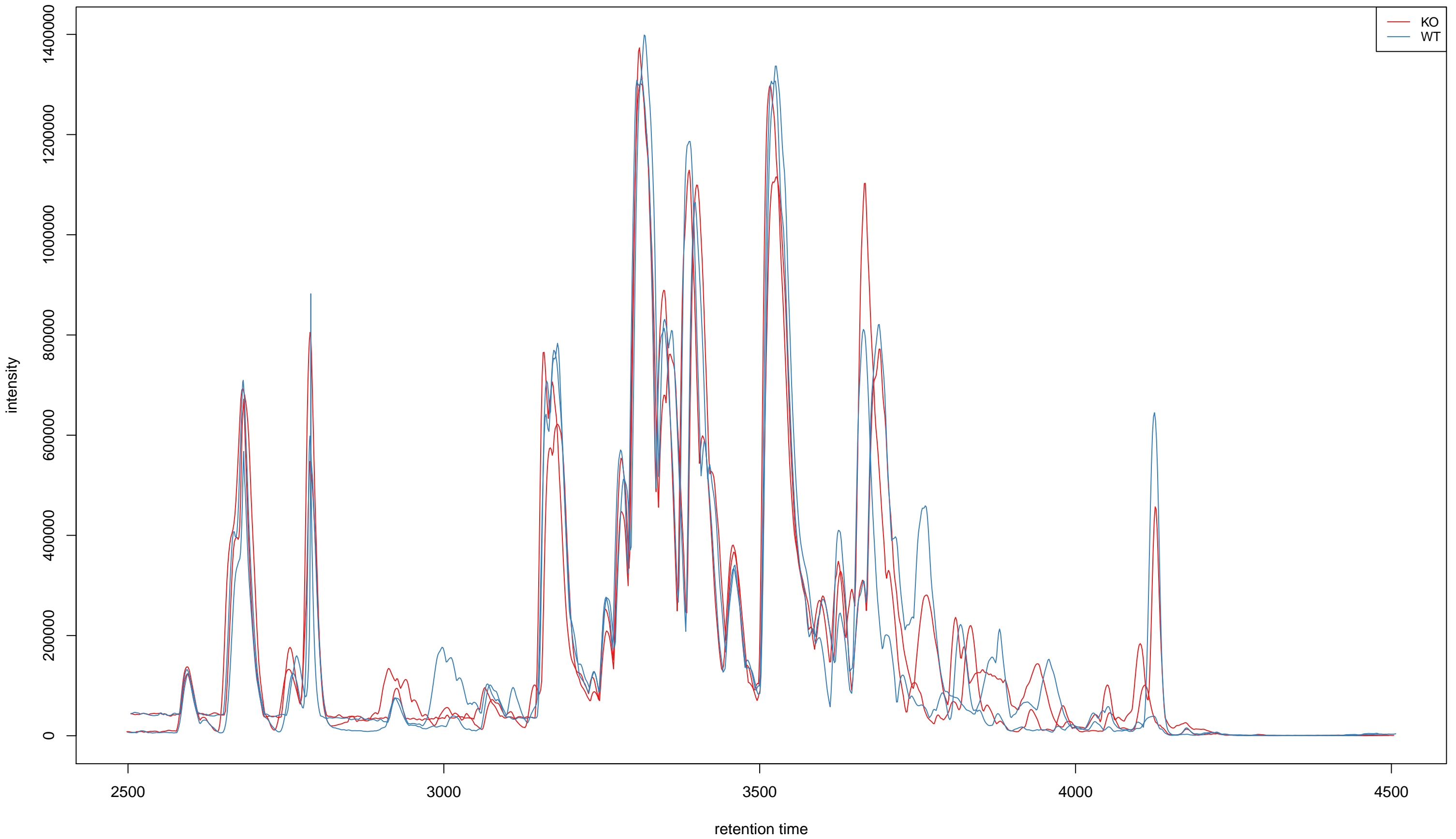
Base Peak Intensity Chromatograms : Adjusted data
