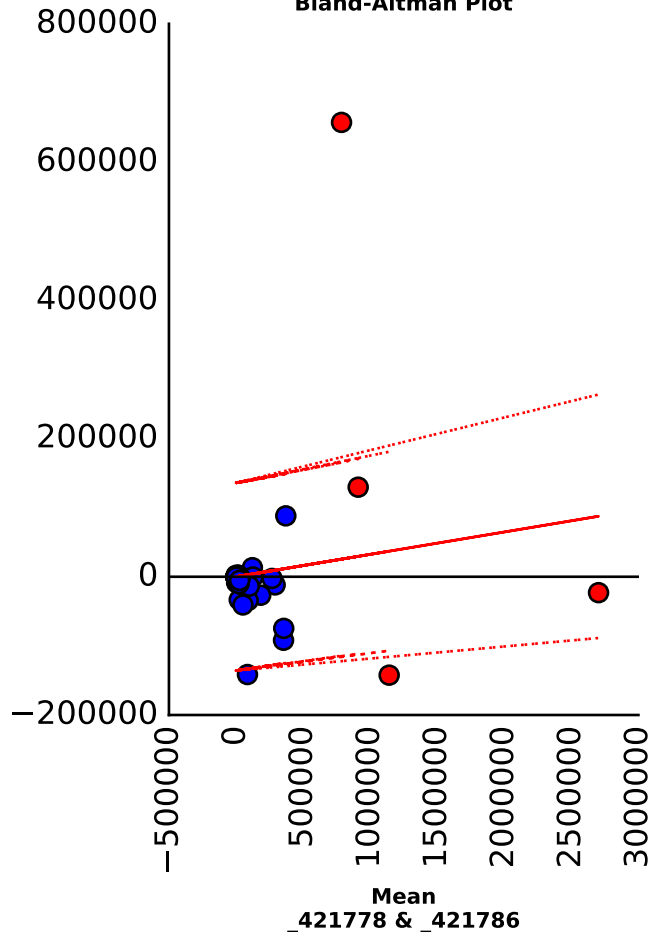
Bland-Altman Plot
