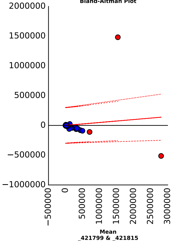
Bland-Altman Plot
