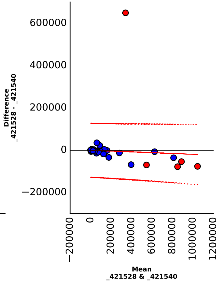
Bland-Altman Plot
