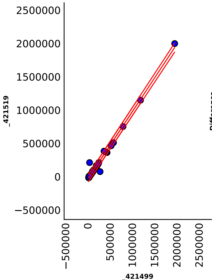
Scatter plot
