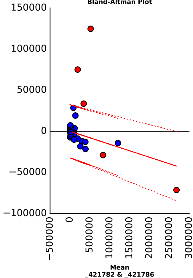
Bland-Altman Plot
