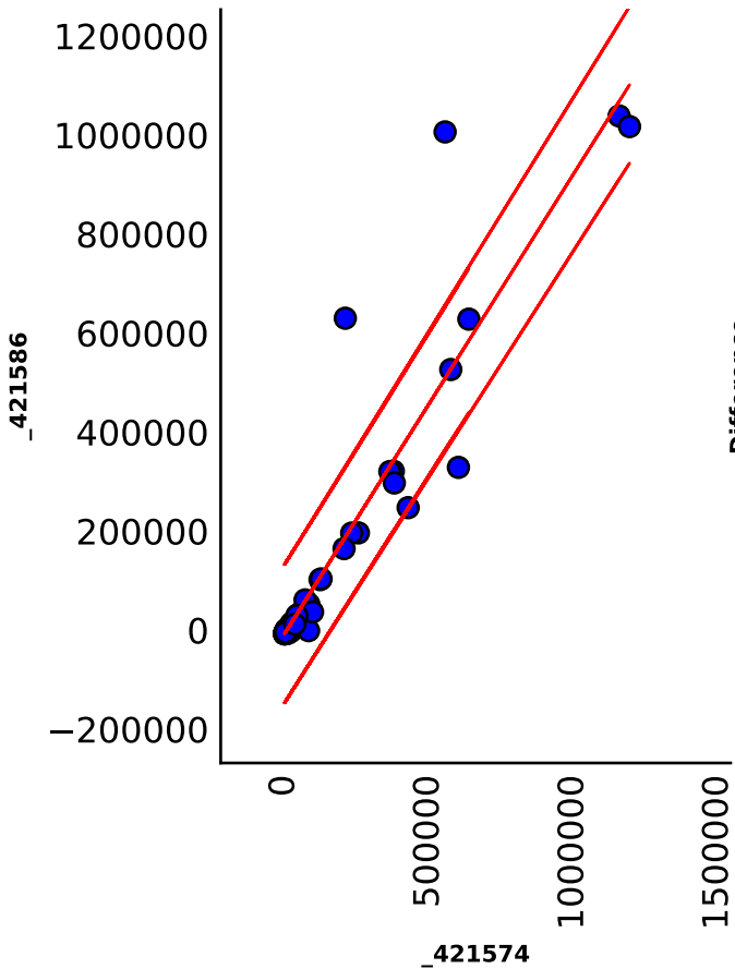
Scatter plot
