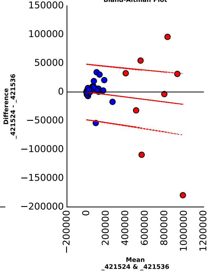
Bland-Altman Plot
