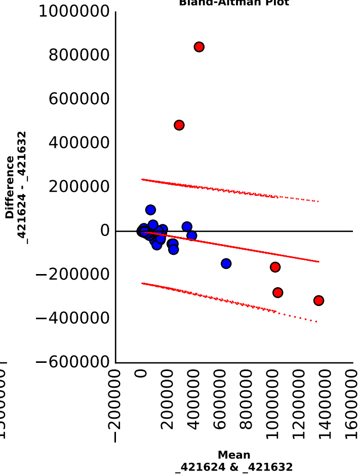
Bland-Altman Plot
