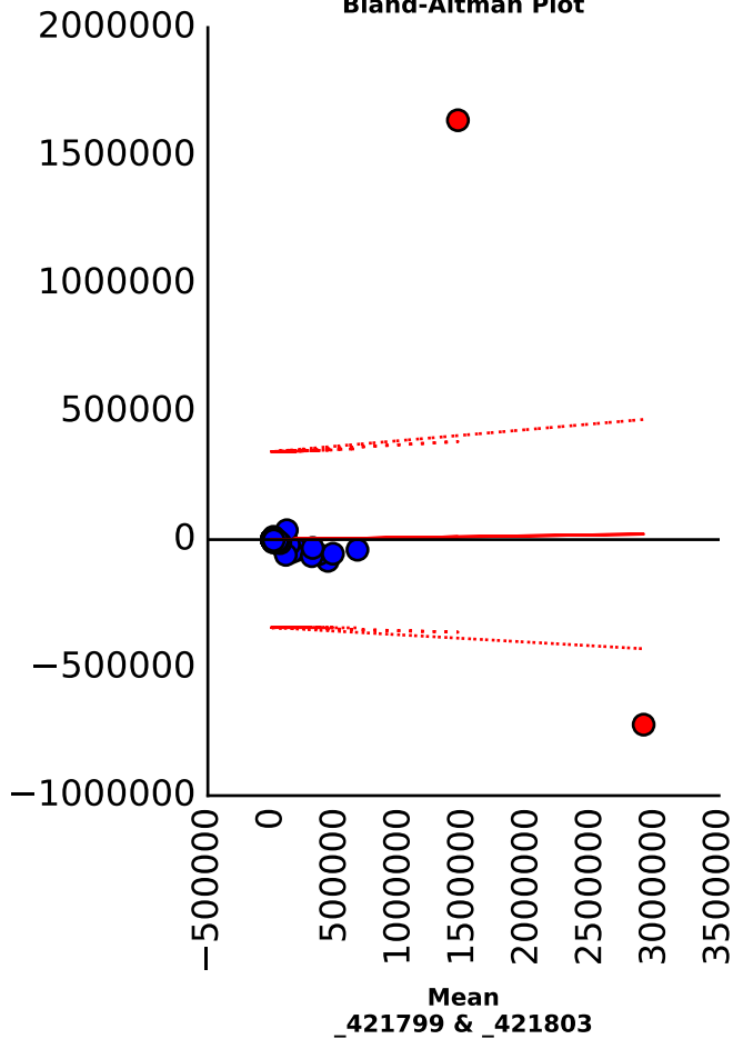
Bland-Altman Plot
