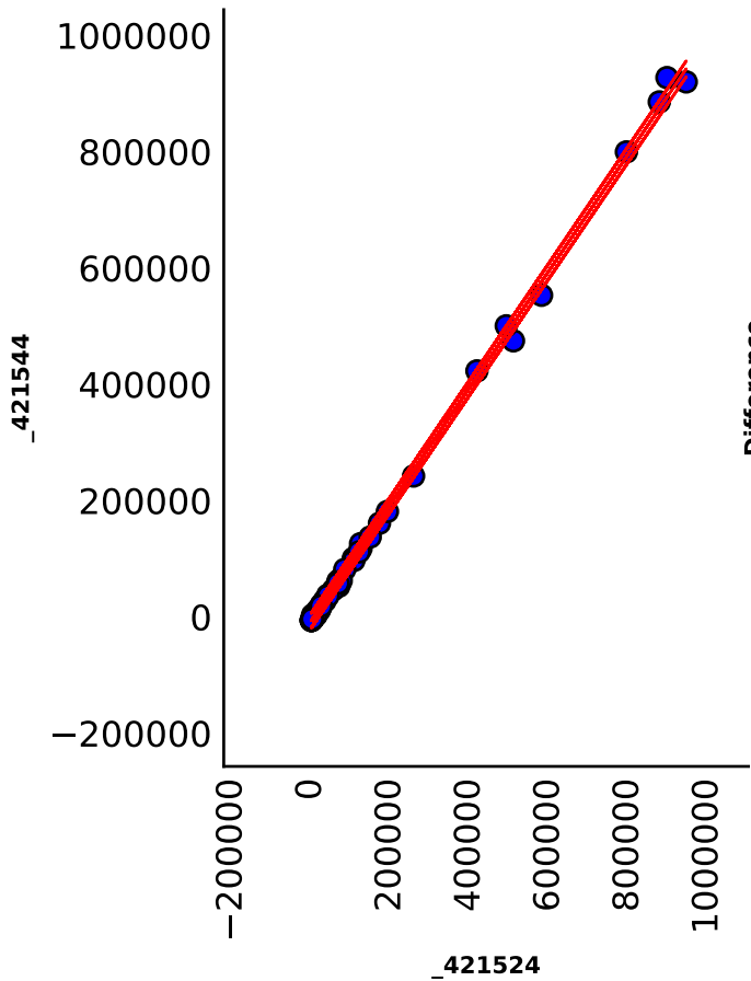
Scatter plot
