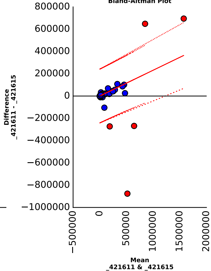
Bland-Altman Plot
