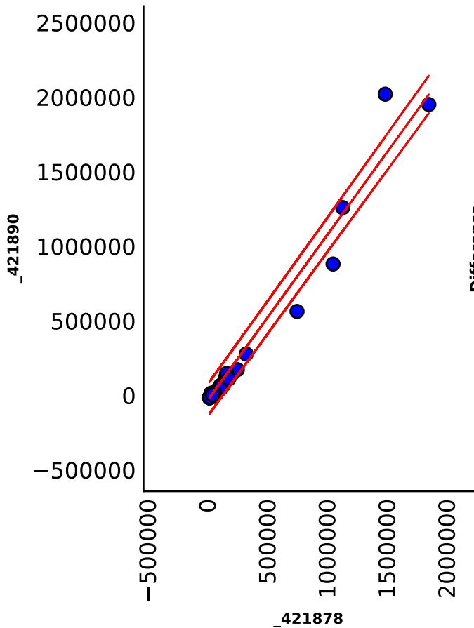
Scatter plot
