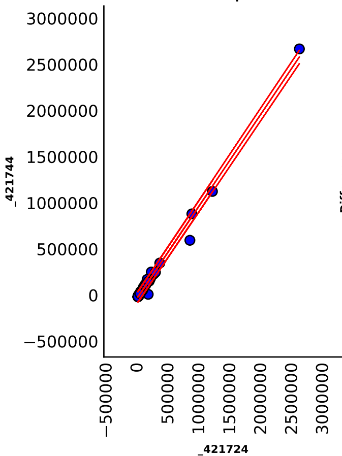
Scatter plot
