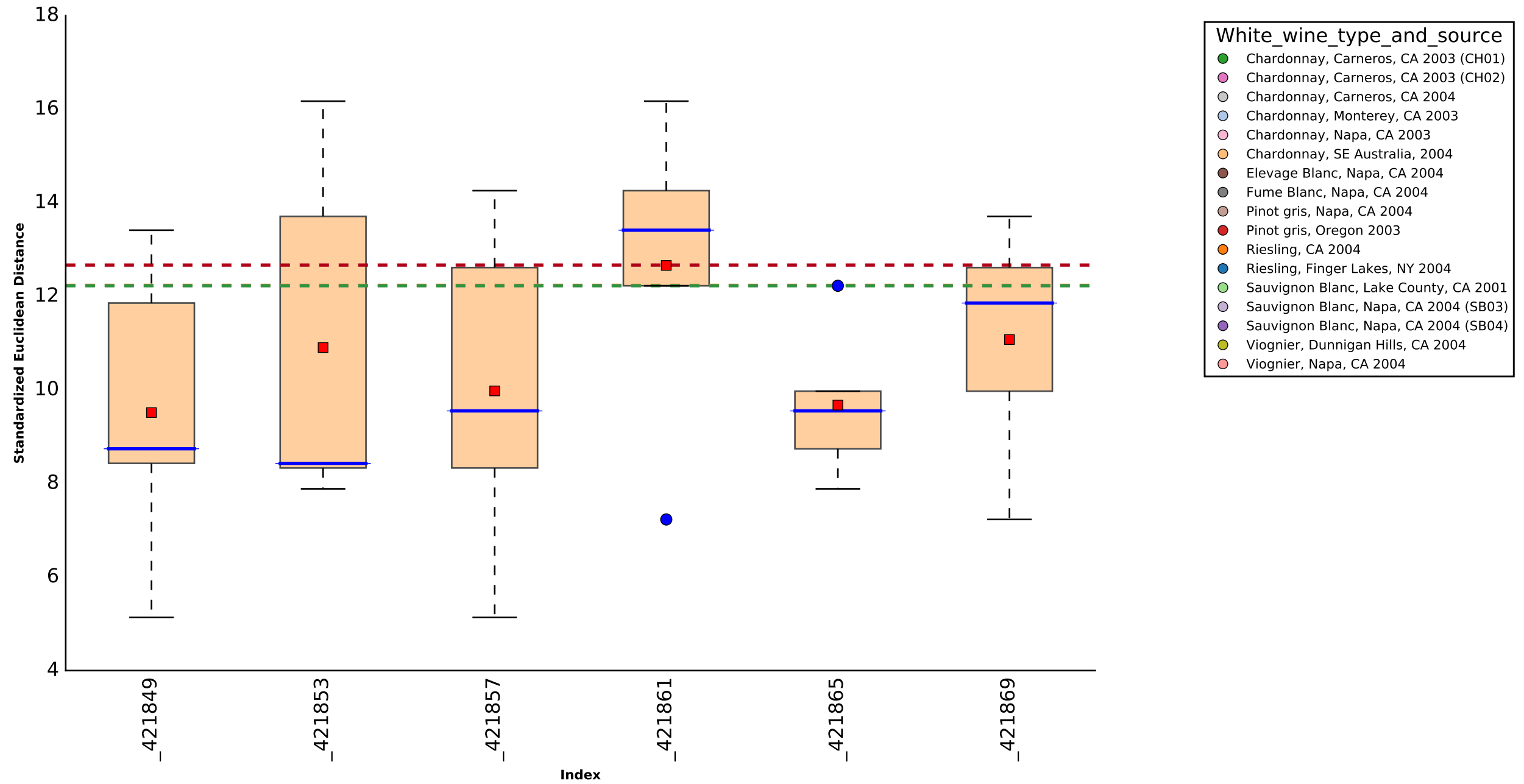
Box-plots for pairwise standardized Euclidean Distance from samples in group Chardonnay, SE Australia, 2004
