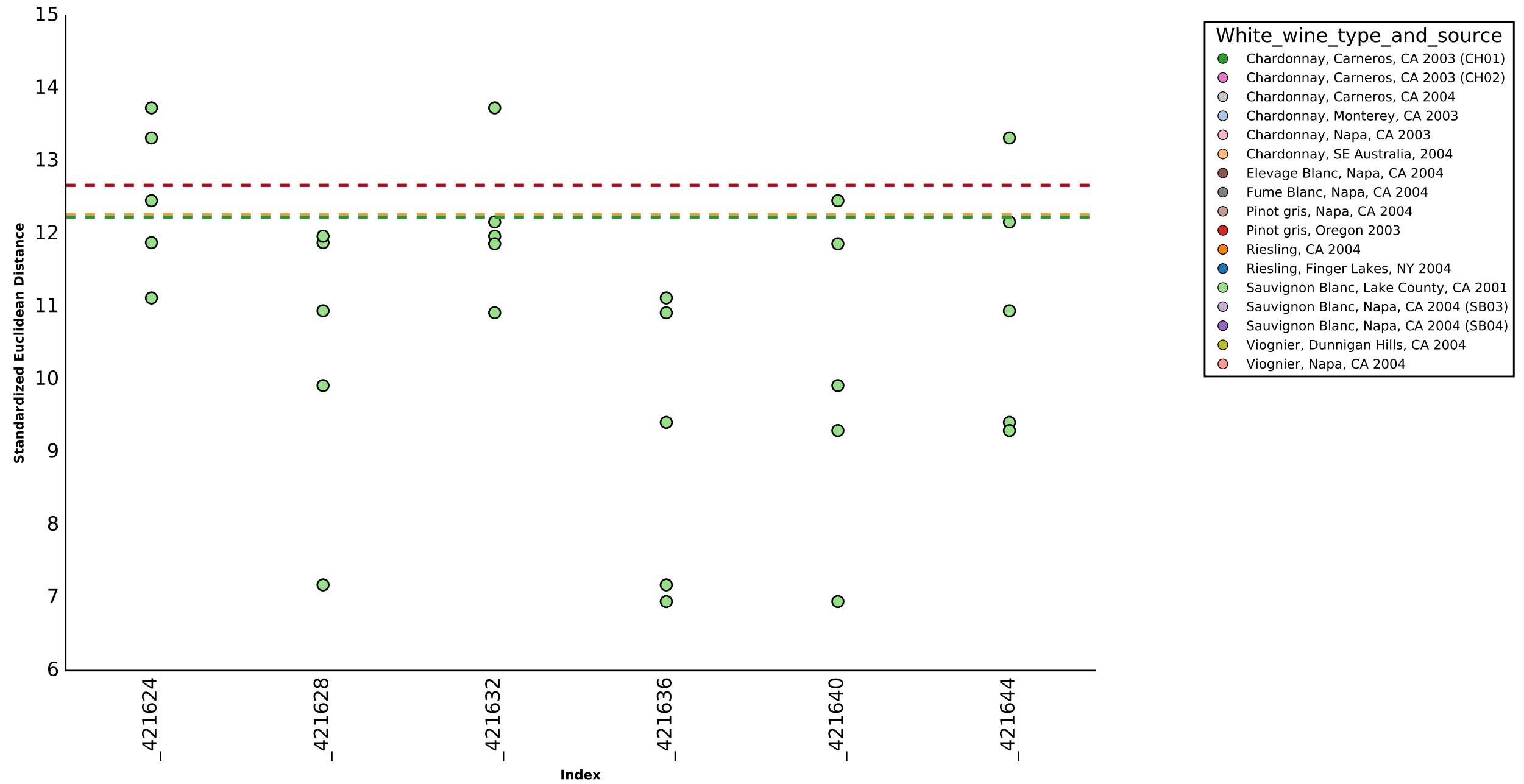
Pairwise standardized Euclidean Distance from samples in group Sauvignon Blanc, Lake County, CA 2001
