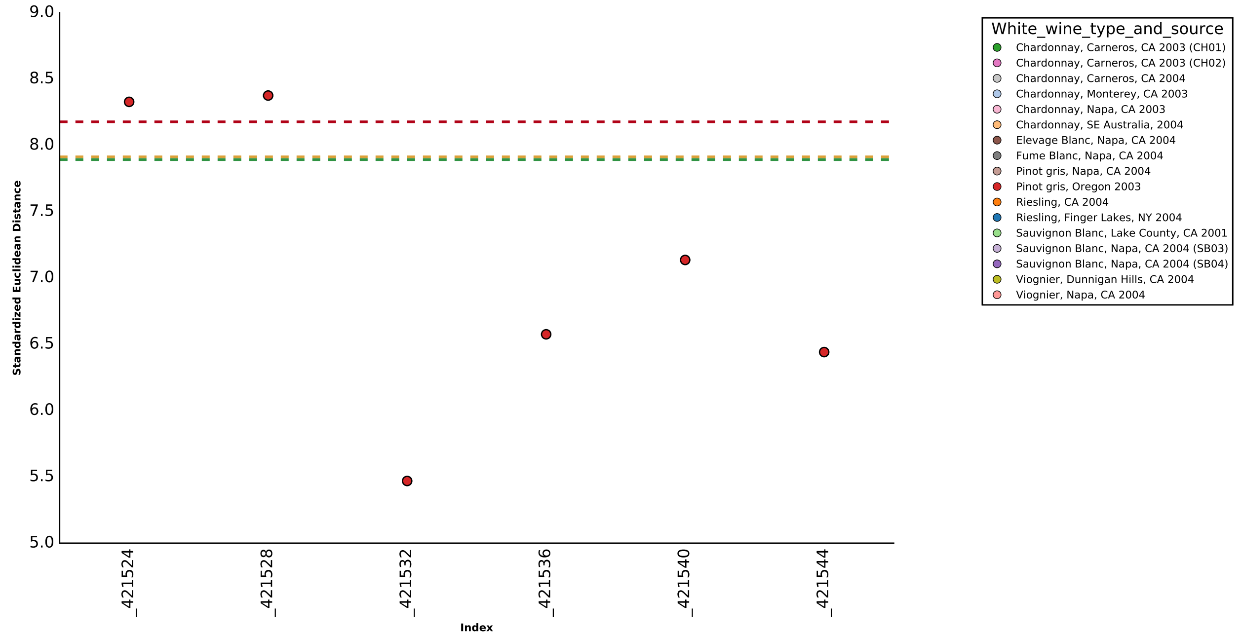
Standardized Euclidean Distance from samples in group Pinot gris, Oregon 2003 to the mean
