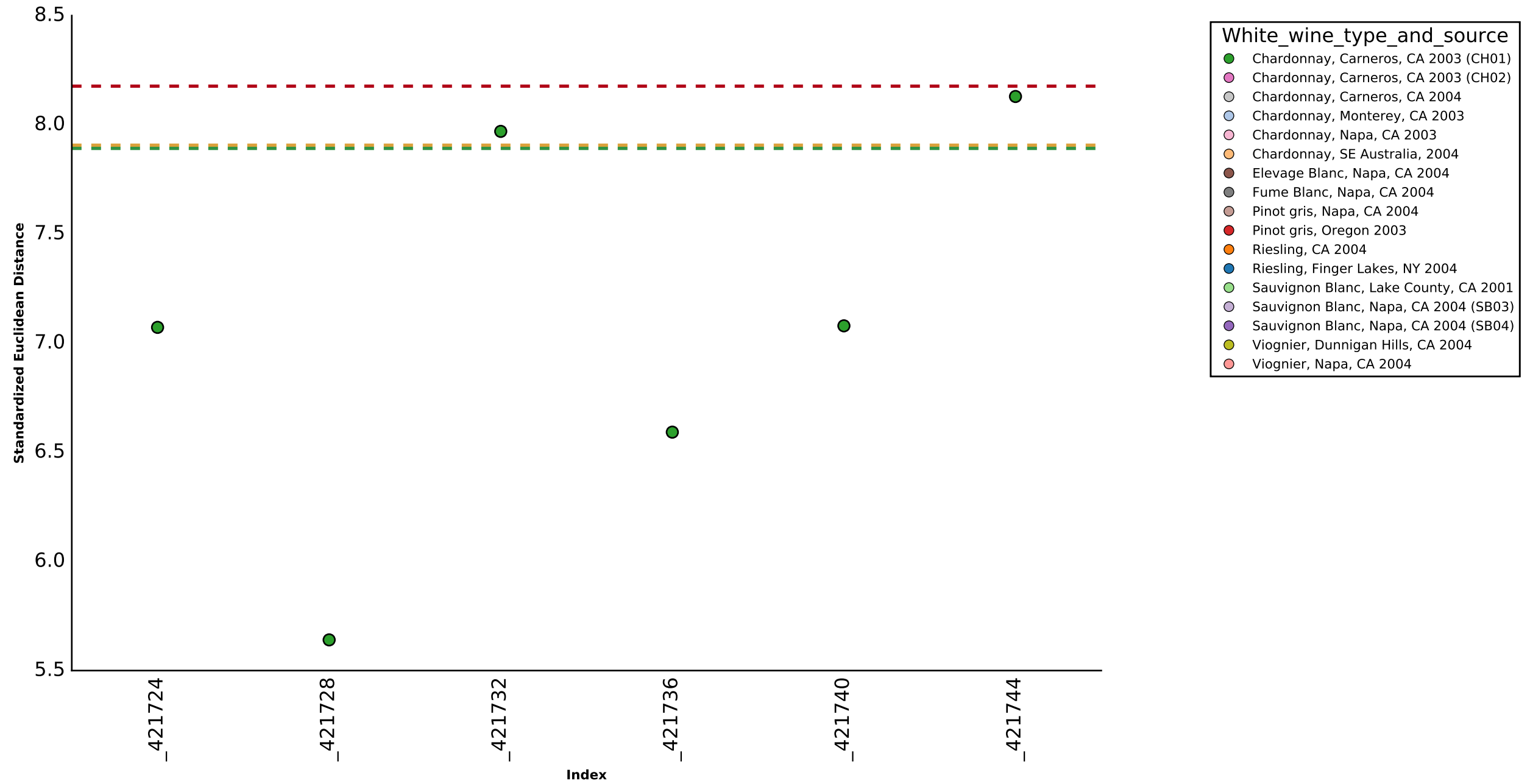
Standardized Euclidean Distance from samples in group Chardonnay, Carneros, CA 2003 (CH01) to the mean
