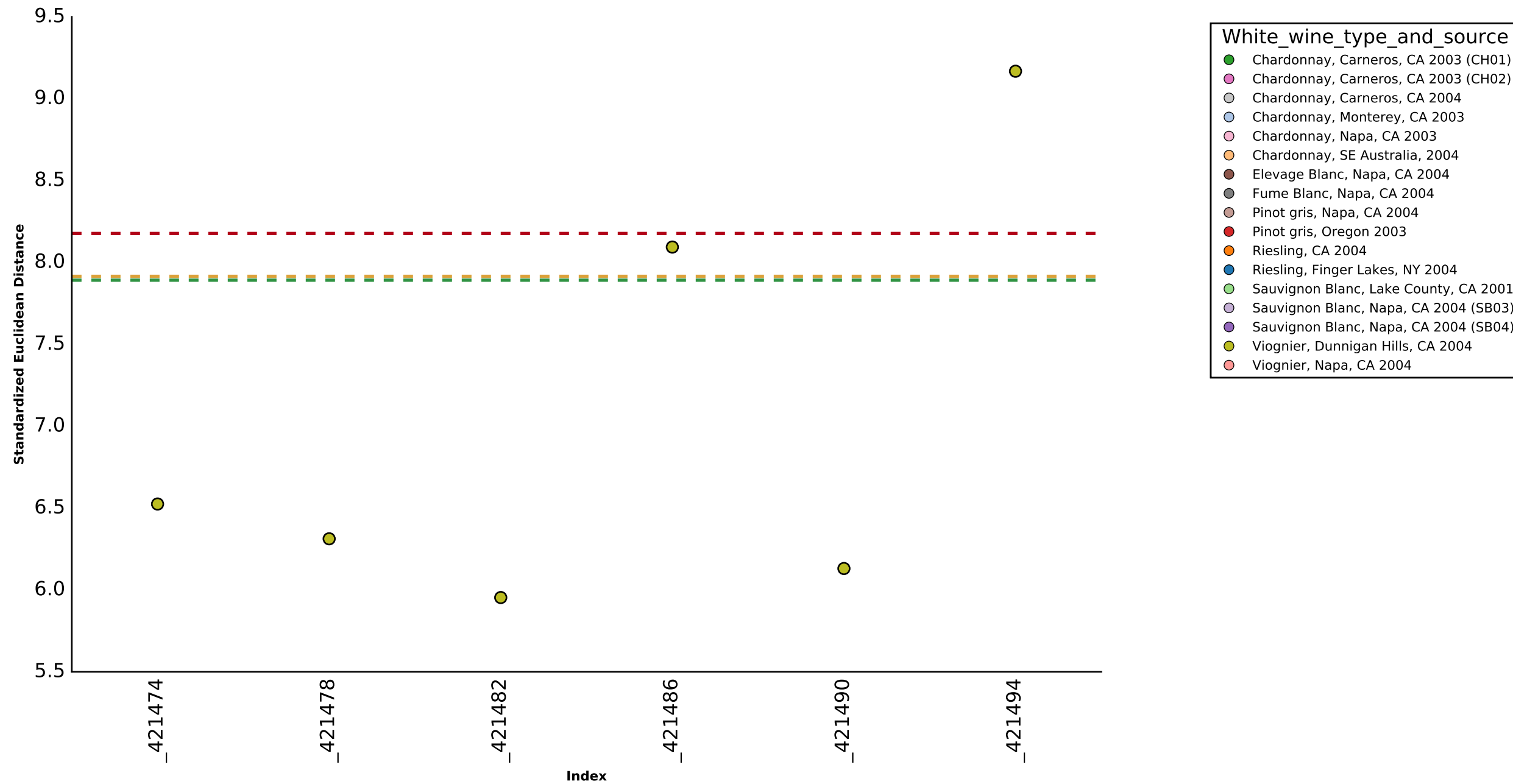
Standardized Euclidean Distance from samples in group Viognier, Dunnigan Hills, CA 2004 to the mean
