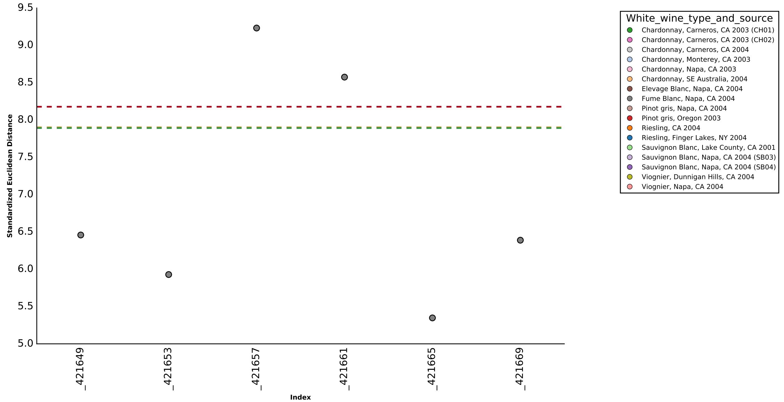
Standardized Euclidean Distance from samples in group Fume Blanc, Napa, CA 2004 to the mean
