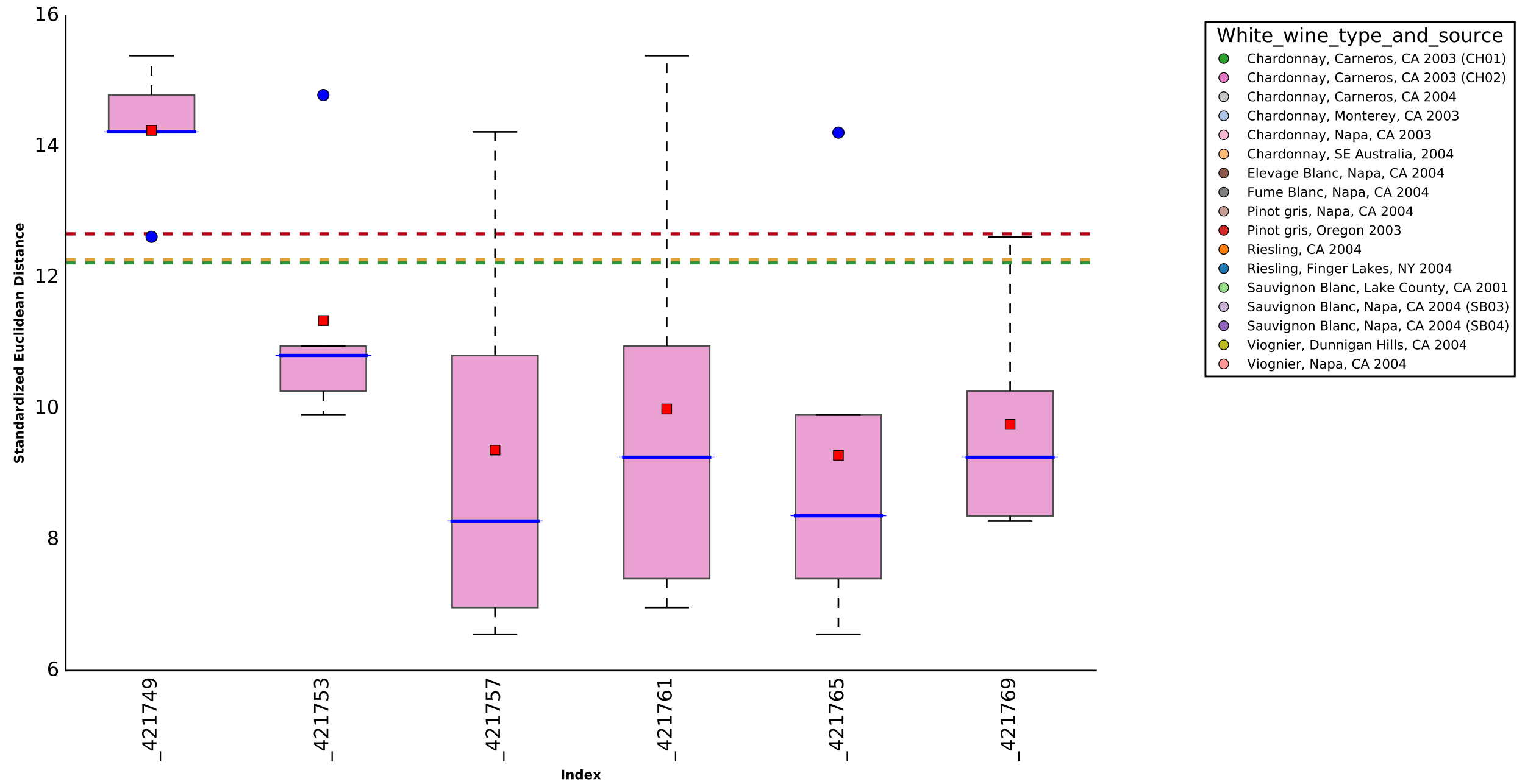
Box-plots for pairwise standardized Euclidean Distance from samples in group Chardonnay, Carneros, CA 2003 (CH2)
