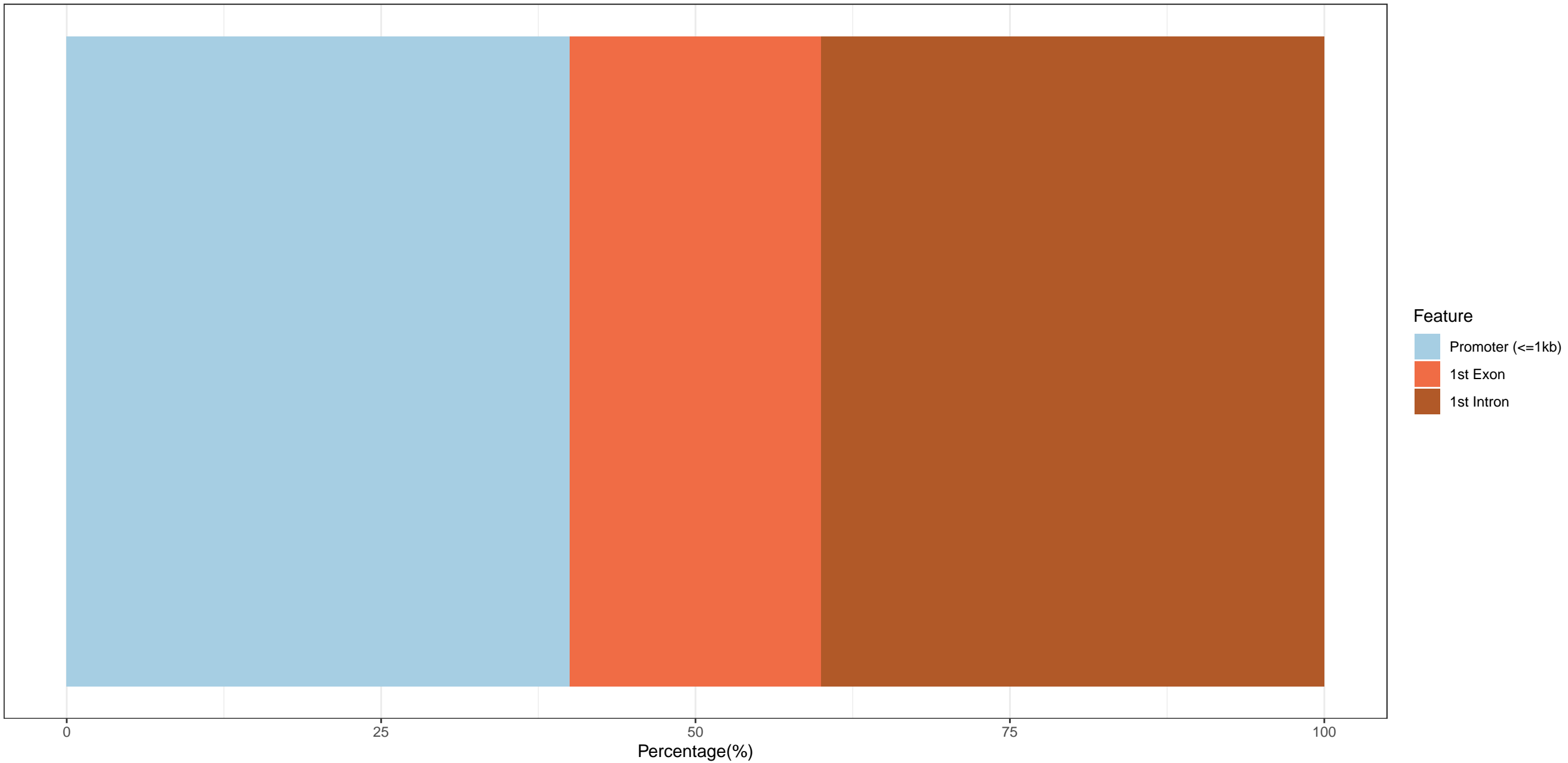
Feature Distribution
